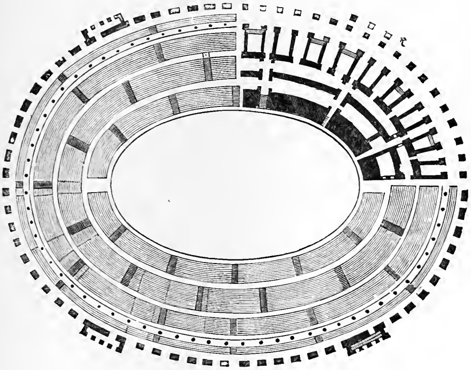
FIG. 131.—PLAN OF THE COLOSSEUM, ROME.
